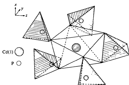
Fig. 2. Polyhedral environment of Cd(1) in Cd_4Na(PO_4)_3 .
