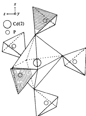
Fig. 3. Polyhedral environment of Cd(2) in Cd_4Na(PO_4)_3 .
