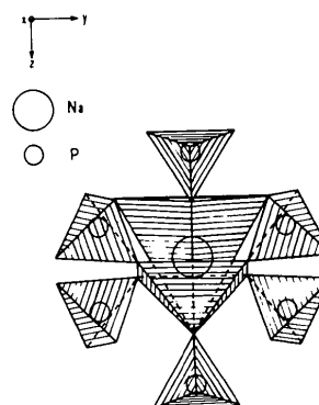
Fig. 4. Coordination polyhedron of Na in Cd_4Na(PO_4)_3 .
